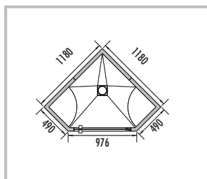
■ MODUL-CAB-F 1180 pentagonal, 2 x bench form SOLO quadrant
