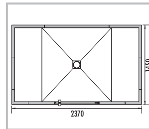
■ MODUL-CAB-R 2370/1450 rectangular, 2 x bench form SOLO
